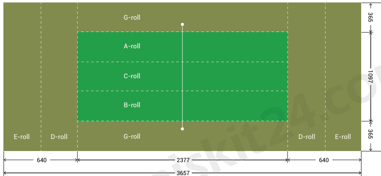
ROLLS LAYOUT*
